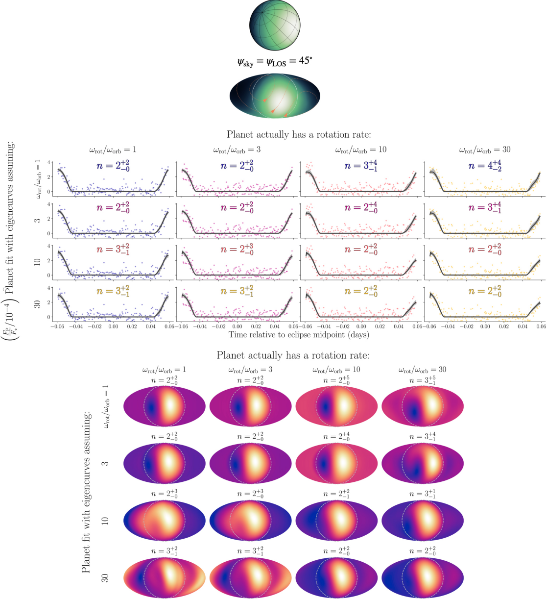
Figure 15. from Arthur D. Adams and Emily Rauscher 2023 Astron. J. 165 doi:10.3847/1538-3881/ac9f46 https://dx.doi.org/10.3847/1538-3881/ac9f46 © 2022. The Author(s). Published by the American Astronomical Society.
