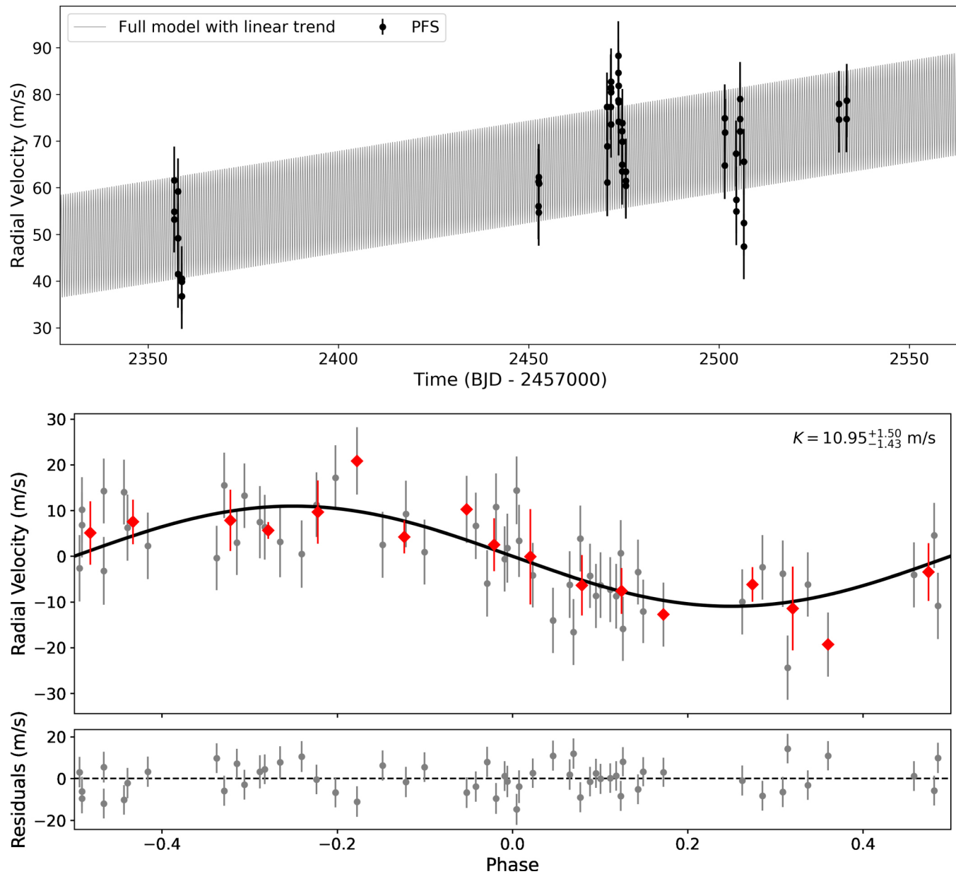
Figure 7. from Zahra Essack et al 2023 Astron. J. 165 doi:10.3847/1538-3881/ac9c5b https://dx.doi.org/10.3847/1538-3881/ac9c5b © 2023. The Author(s). Published by the American Astronomical Society.
