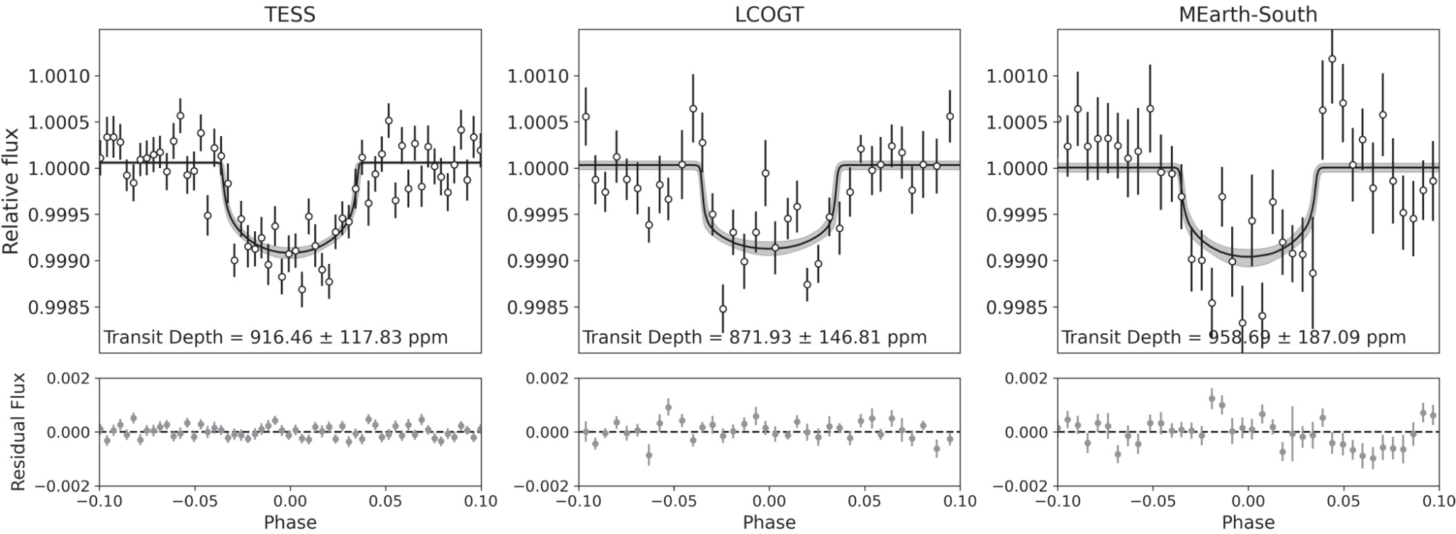
Figure 5. from Zahra Essack et al 2023 Astron. J. 165 doi:10.3847/1538-3881/ac9c5b https://dx.doi.org/10.3847/1538-3881/ac9c5b © 2023. The Author(s). Published by the American Astronomical Society.
