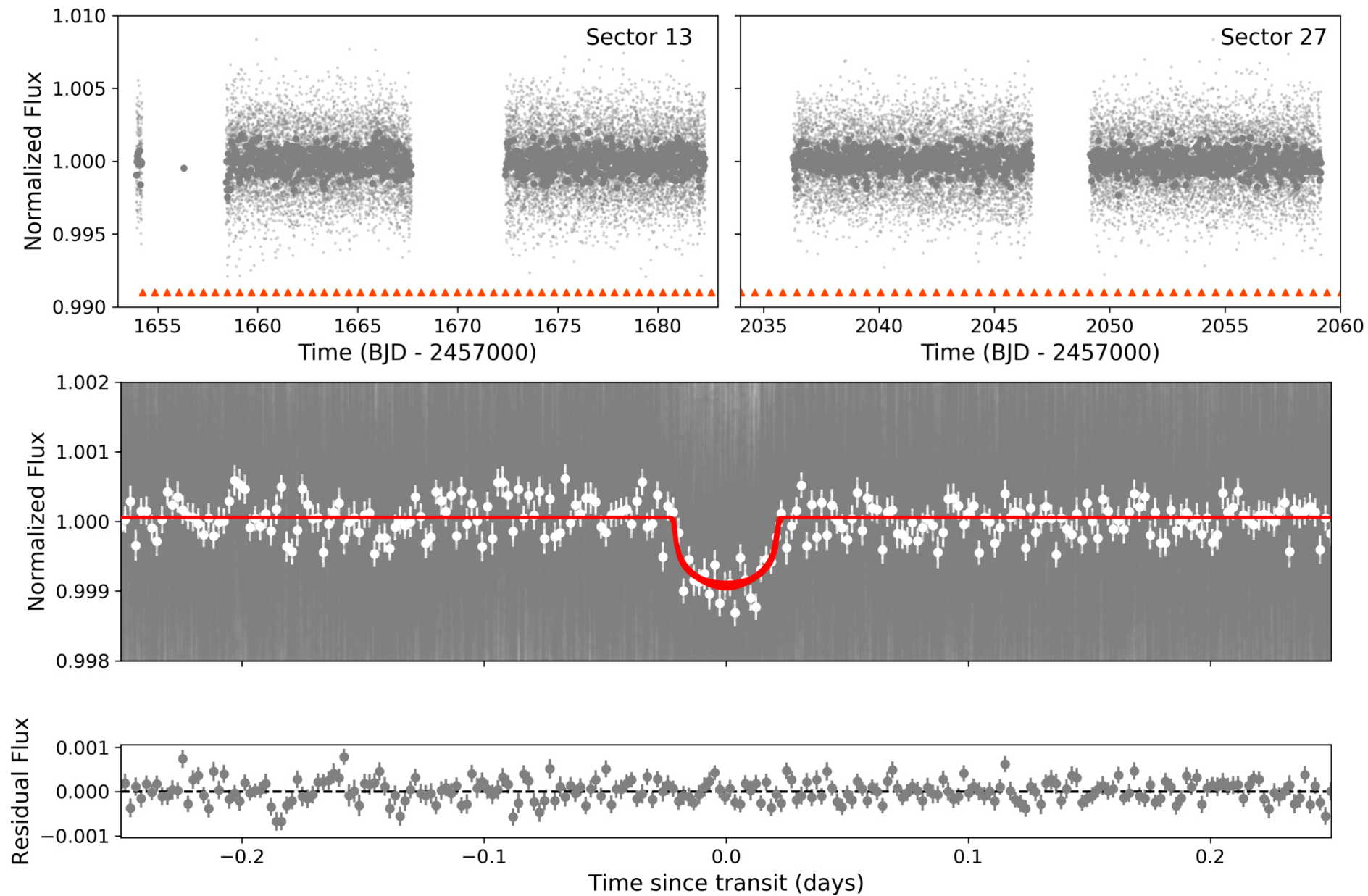
Figure 4. from Zahra Essack et al 2023 Astron. J. 165 doi:10.3847/1538-3881/ac9c5b https://dx.doi.org/10.3847/1538-3881/ac9c5b © 2023. The Author(s). Published by the American Astronomical Society.
