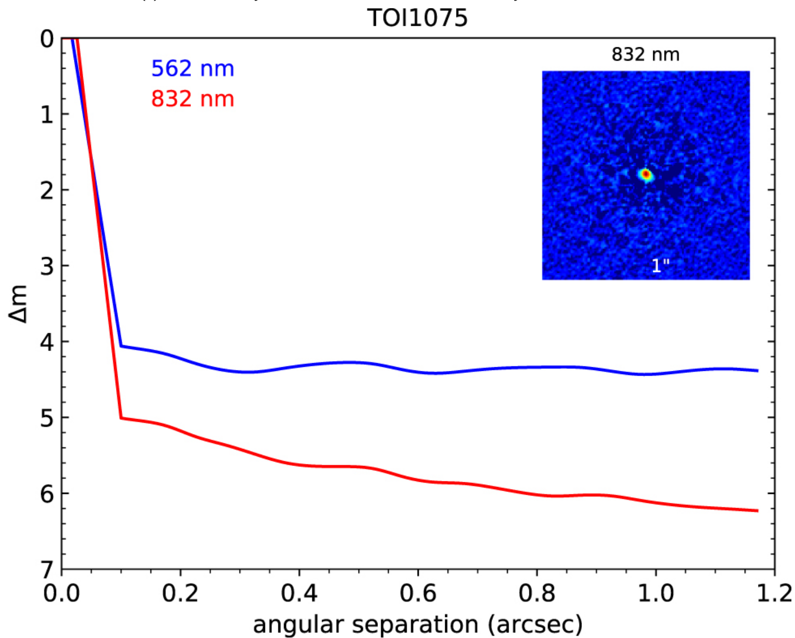
Figure 2. from Zahra Essack et al 2023 Astron. J. 165 doi:10.3847/1538-3881/ac9c5b https://dx.doi.org/10.3847/1538-3881/ac9c5b © 2023. The Author(s). Published by the American Astronomical Society.
