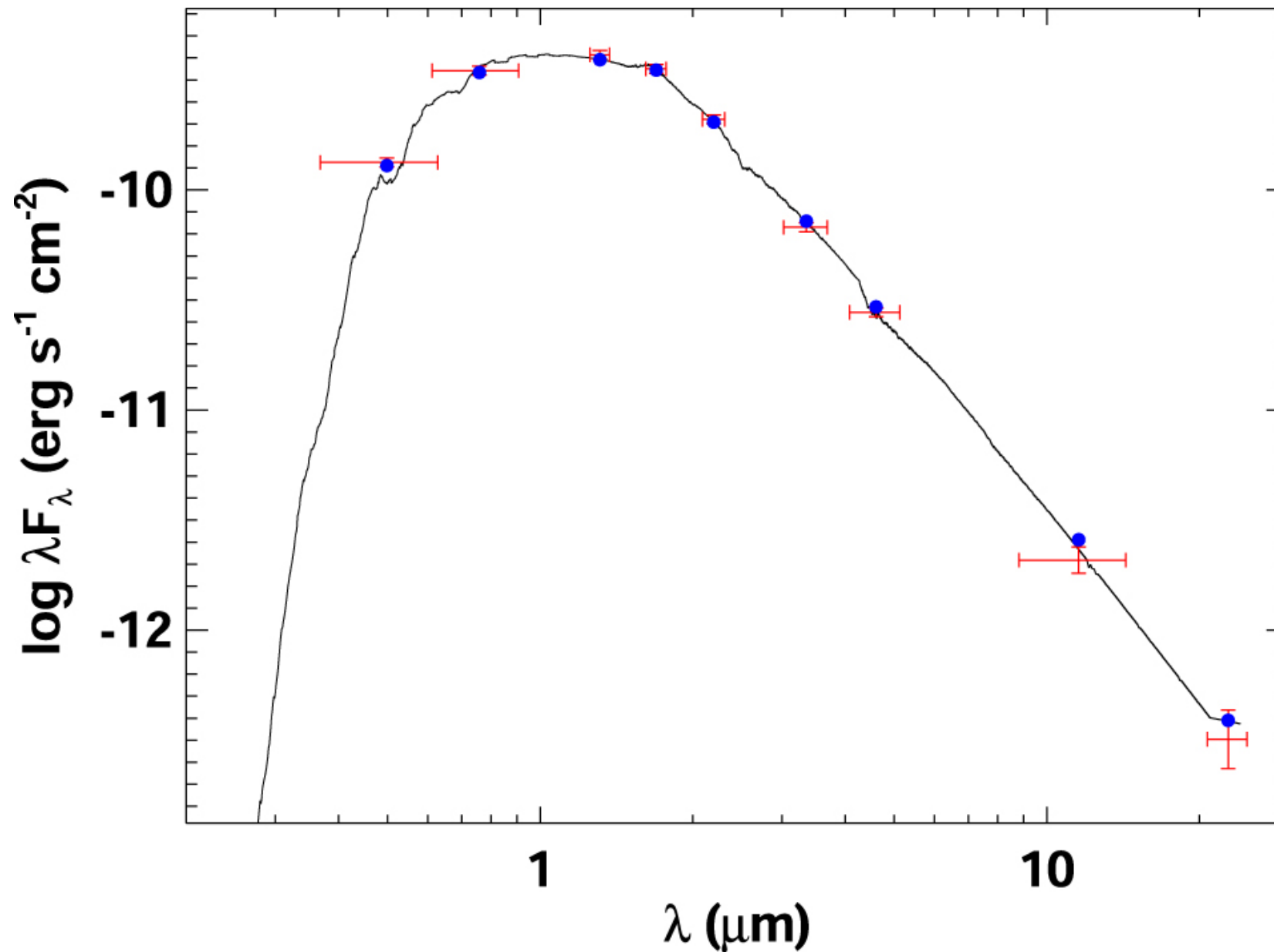
Figure 1. from Zahra Essack et al 2023 Astron. J. 165 doi:10.3847/1538-3881/ac9c5b https://dx.doi.org/10.3847/1538-3881/ac9c5b © 2023. The Author(s). Published by the American Astronomical Society.
