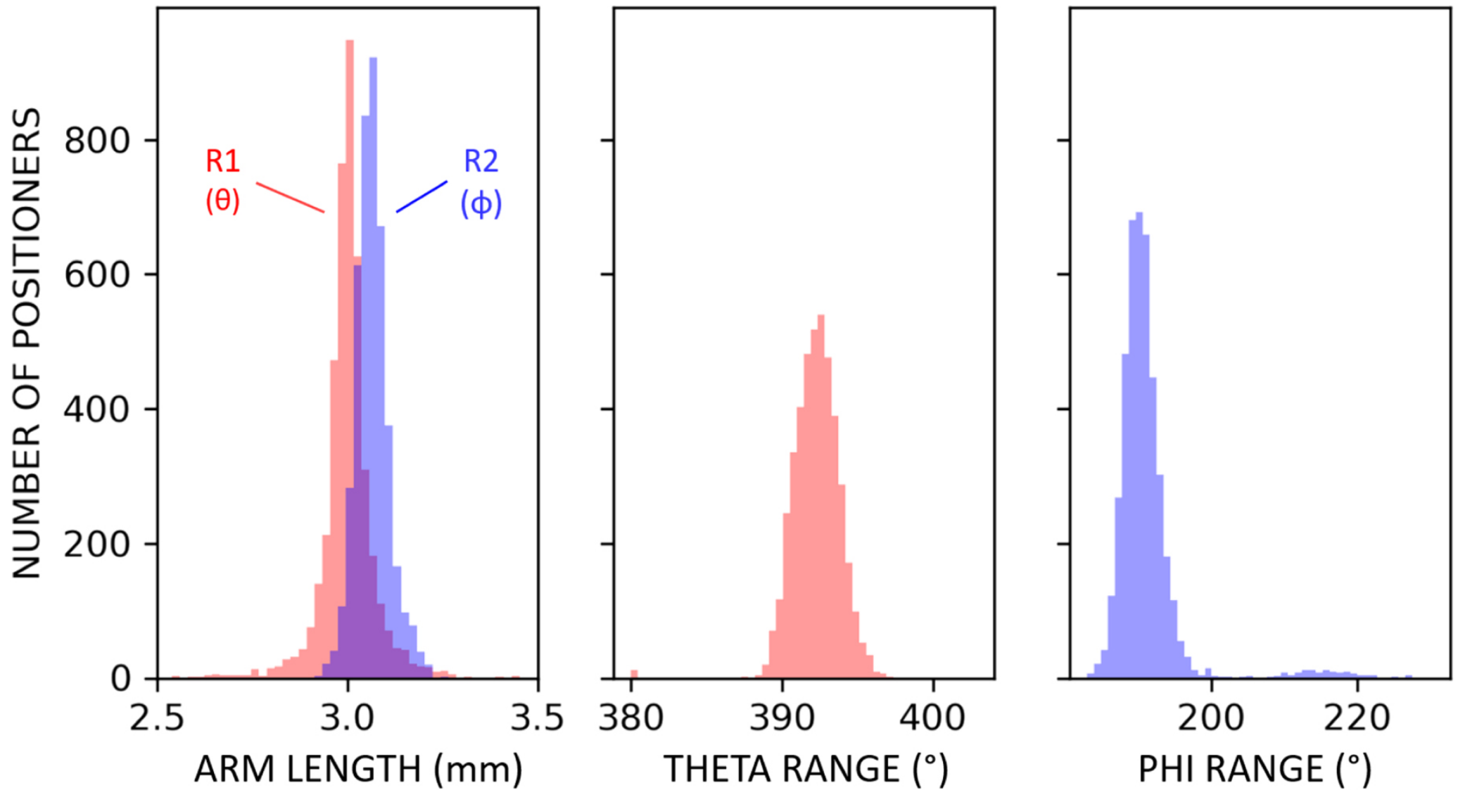
Figure 7. from Joseph Harry Silber et al 2023 Astron. J. 165 doi:10.3847/1538-3881/ac9ab1 https://dx.doi.org/10.3847/1538-3881/ac9ab1 © 2022. The Author(s). Published by the American Astronomical Society.
