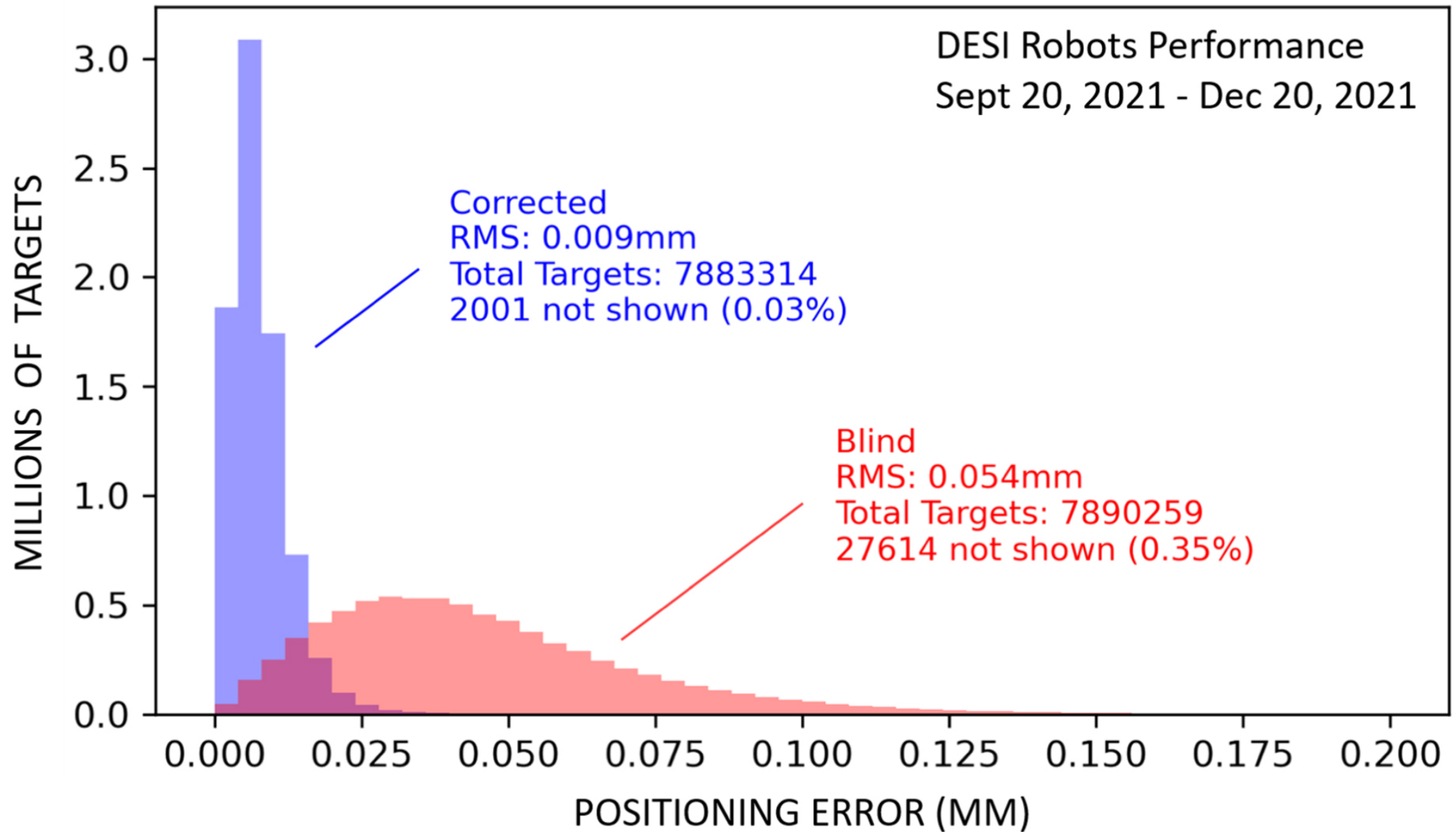
Figure 4. from Joseph Harry Silber et al 2023 Astron. J. 165 doi:10.3847/1538-3881/ac9ab1 https://dx.doi.org/10.3847/1538-3881/ac9ab1 © 2022. The Author(s). Published by the American Astronomical Society.
