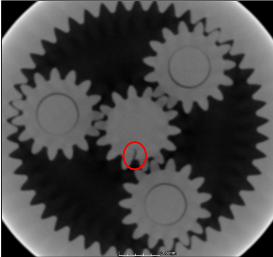
Figure 37. from Joseph Harry Silber et al 2023 Astron. J. 165 doi:10.3847/1538-3881/ac9ab1 https://dx.doi.org/10.3847/1538-3881/ac9ab1 © 2022. The Author(s). Published by the American Astronomical Society.
