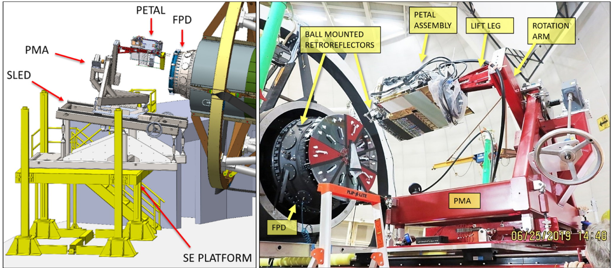
Figure 34. from Joseph Harry Silber et al 2023 Astron. J. 165 doi:10.3847/1538-3881/ac9ab1 https://dx.doi.org/10.3847/1538-3881/ac9ab1 © 2022. The Author(s). Published by the American Astronomical Society.
