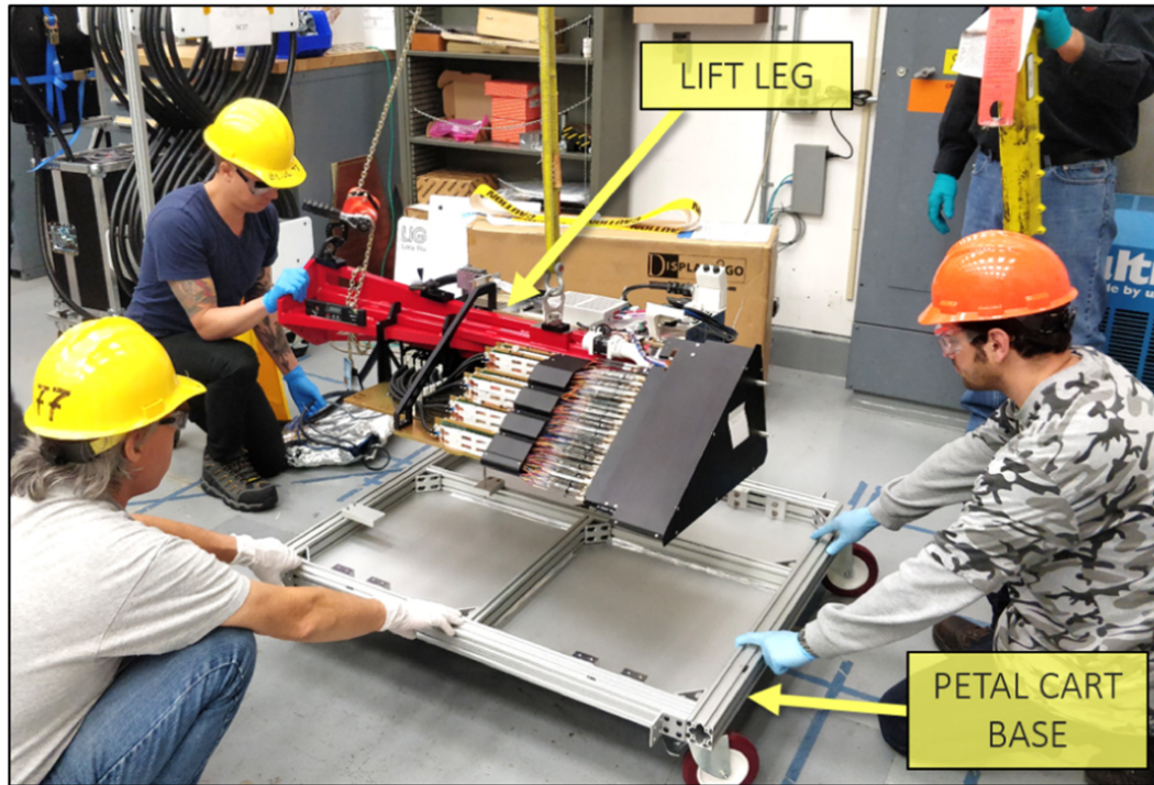
Figure 33. from Joseph Harry Silber et al 2023 Astron. J. 165 doi:10.3847/1538-3881/ac9ab1 https://dx.doi.org/10.3847/1538-3881/ac9ab1 © 2022. The Author(s). Published by the American Astronomical Society.
