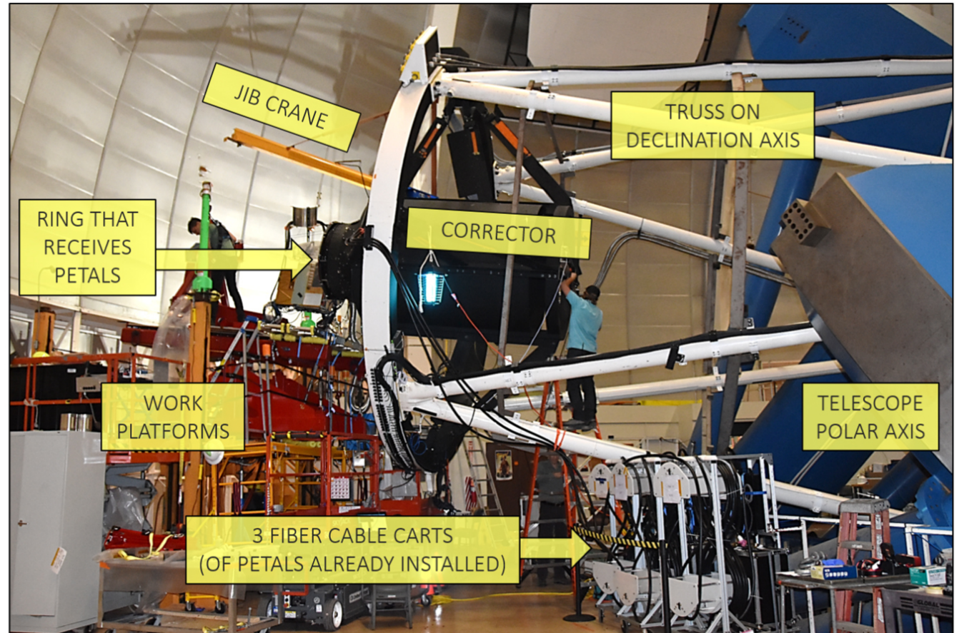
Figure 32. from Joseph Harry Silber et al 2023 Astron. J. 165 doi:10.3847/1538-3881/ac9ab1 https://dx.doi.org/10.3847/1538-3881/ac9ab1 © 2022. The Author(s). Published by the American Astronomical Society.
