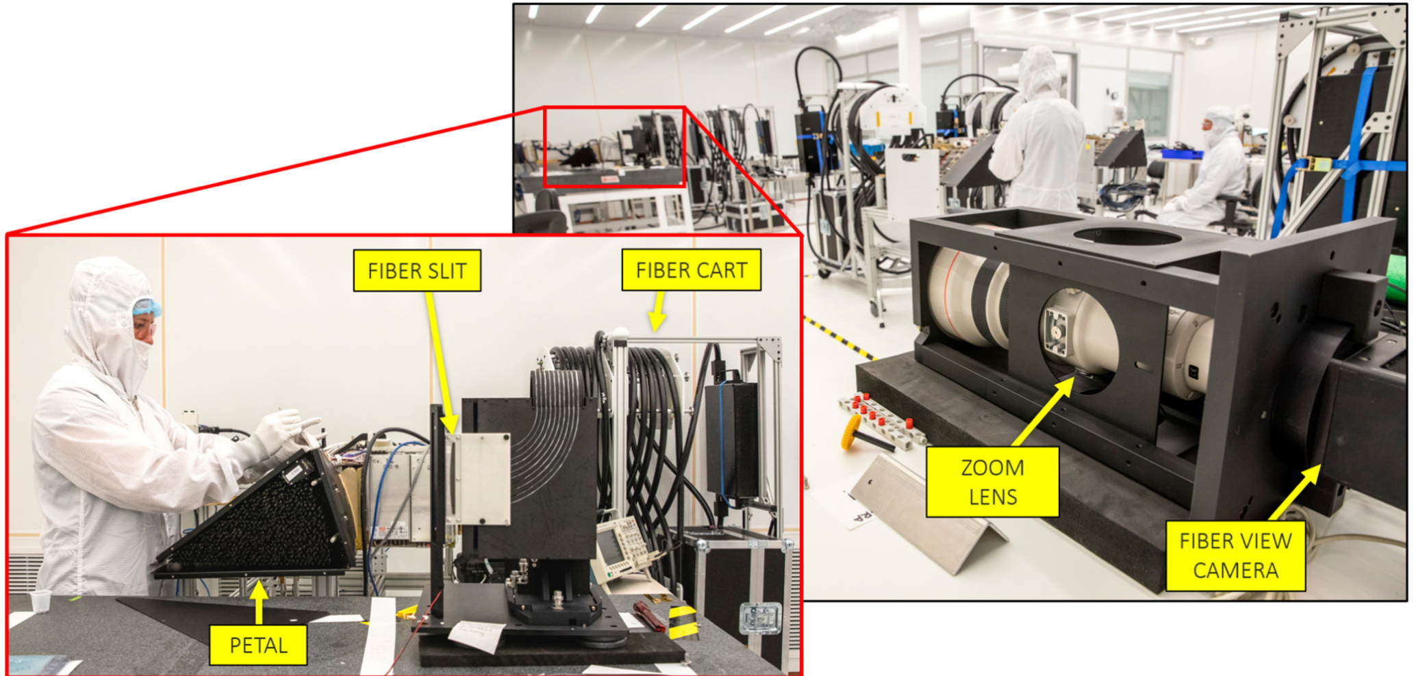
Figure 31. from Joseph Harry Silber et al 2023 Astron. J. 165 doi:10.3847/1538-3881/ac9ab1 https://dx.doi.org/10.3847/1538-3881/ac9ab1 © 2022. The Author(s). Published by the American Astronomical Society.
