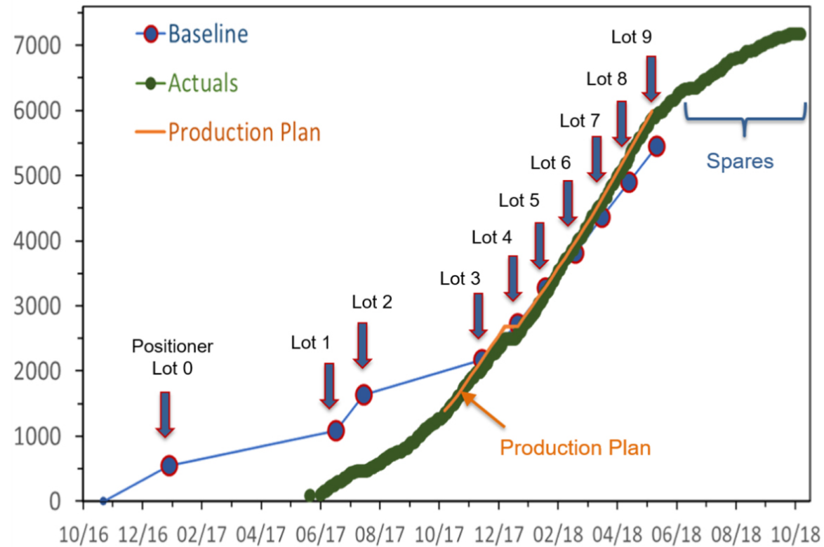
Figure 30. from Joseph Harry Silber et al 2023 Astron. J. 165 doi:10.3847/1538-3881/ac9ab1 https://dx.doi.org/10.3847/1538-3881/ac9ab1 © 2022. The Author(s). Published by the American Astronomical Society.
