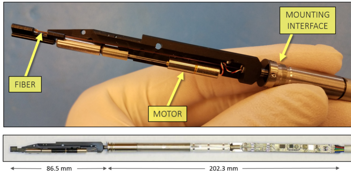
Figure 3. from Joseph Harry Silber et al 2023 Astron. J. 165 doi:10.3847/1538-3881/ac9ab1 https://dx.doi.org/10.3847/1538-3881/ac9ab1 © 2022. The Author(s). Published by the American Astronomical Society.
