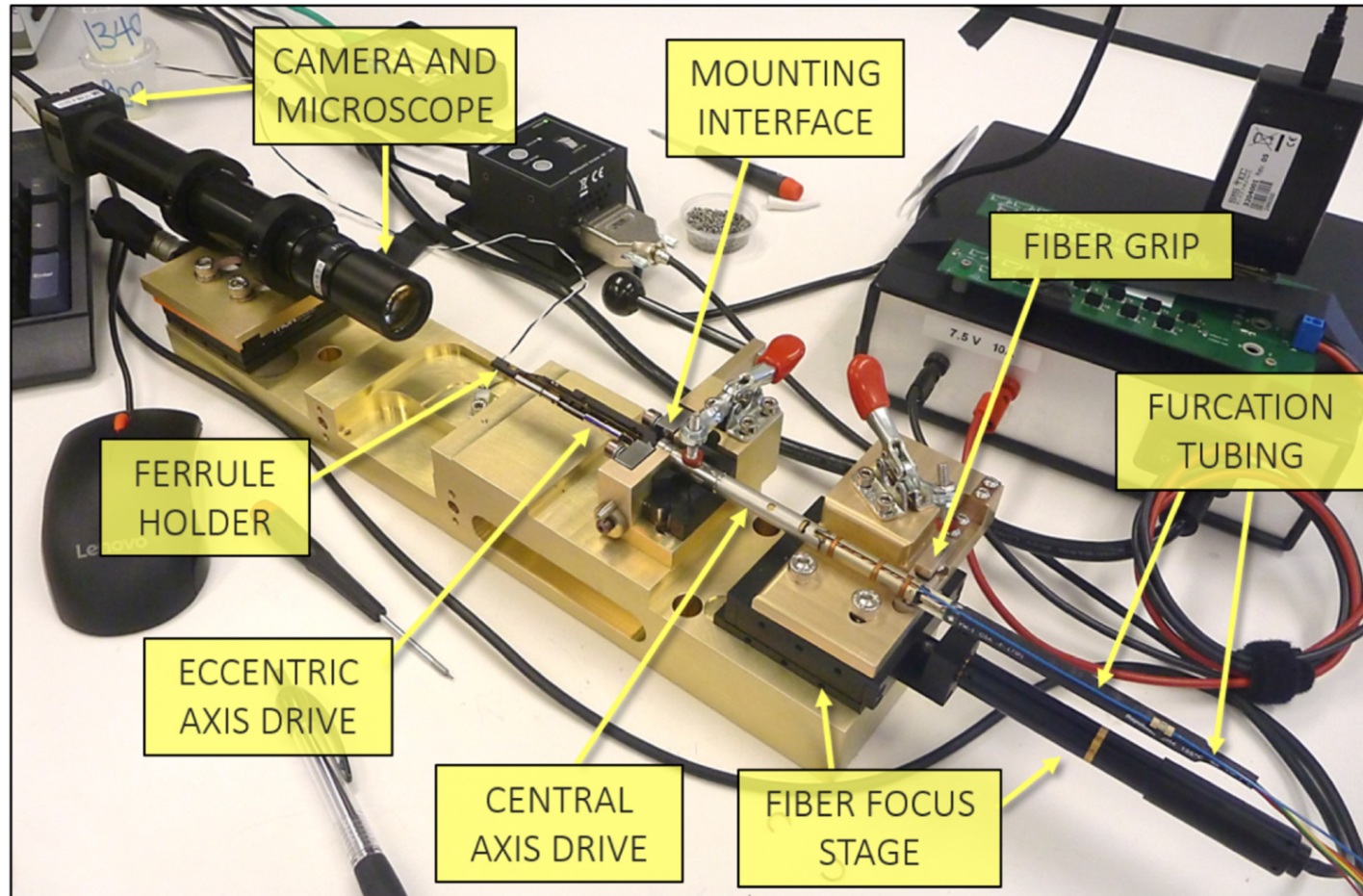
Figure 29. from Joseph Harry Silber et al 2023 Astron. J. 165 doi:10.3847/1538-3881/ac9ab1 https://dx.doi.org/10.3847/1538-3881/ac9ab1 © 2022. The Author(s). Published by the American Astronomical Society.
