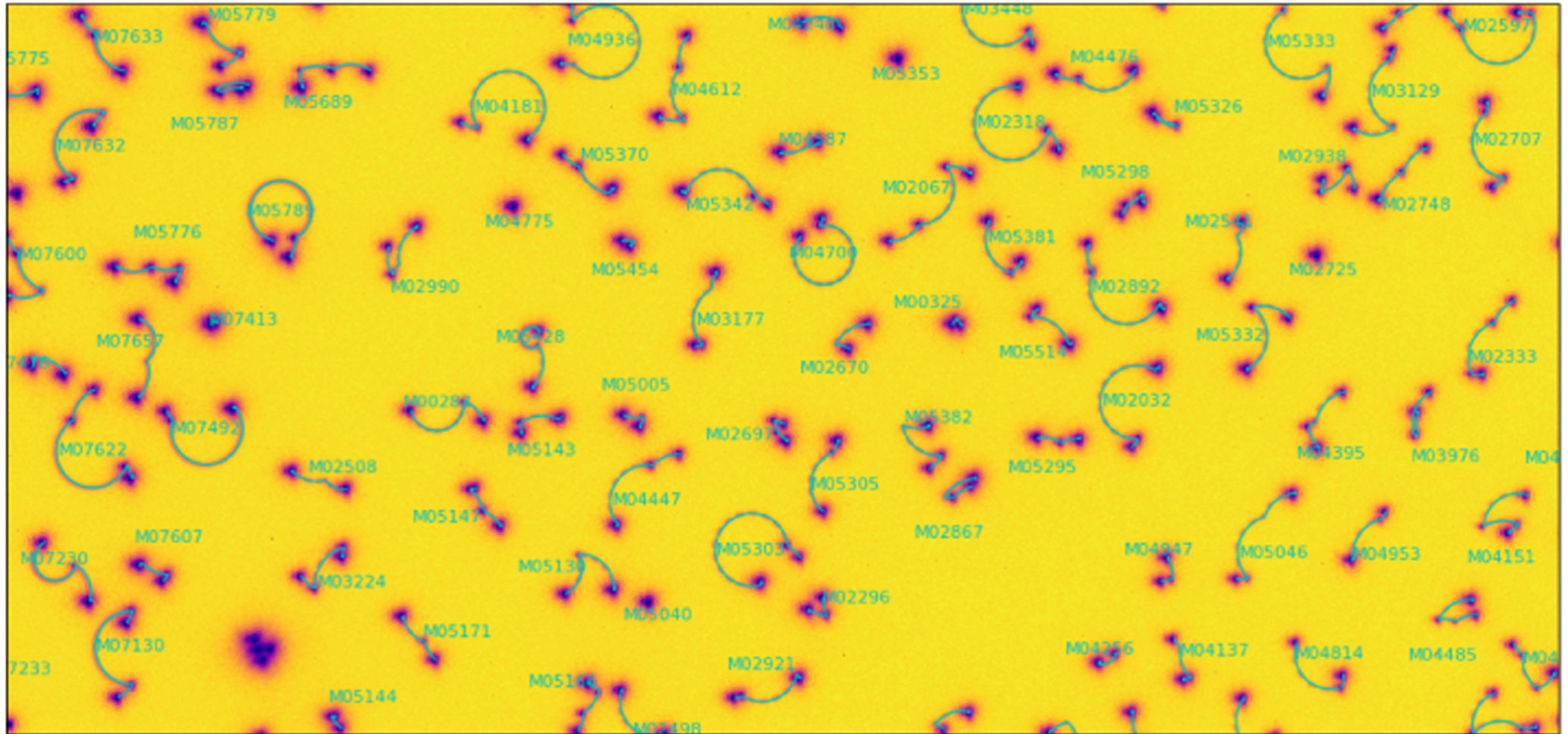
Figure 25. from Joseph Harry Silber et al 2023 Astron. J. 165 doi:10.3847/1538-3881/ac9ab1 https://dx.doi.org/10.3847/1538-3881/ac9ab1 © 2022. The Author(s). Published by the American Astronomical Society.
