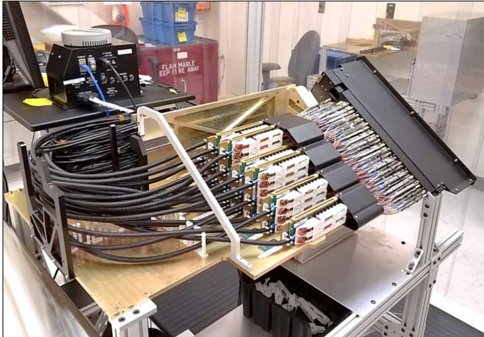
Figure 24. from Joseph Harry Silber et al 2023 Astron. J. 165 doi:10.3847/1538-3881/ac9ab1 https://dx.doi.org/10.3847/1538-3881/ac9ab1 © 2022. The Author(s). Published by the American Astronomical Society.
