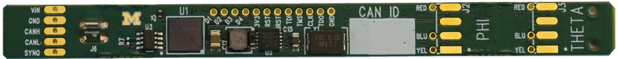
Figure 23. from Joseph Harry Silber et al 2023 Astron. J. 165 doi:10.3847/1538-3881/ac9ab1 https://dx.doi.org/10.3847/1538-3881/ac9ab1 © 2022. The Author(s). Published by the American Astronomical Society.
