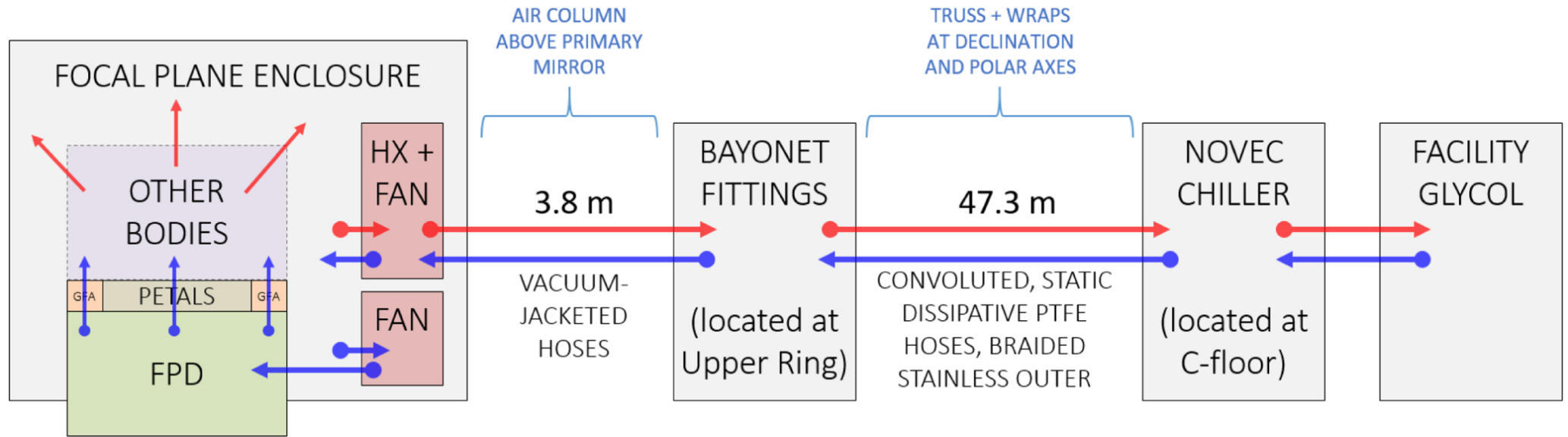
Figure 21. from Joseph Harry Silber et al 2023 Astron. J. 165 doi:10.3847/1538-3881/ac9ab1 https://dx.doi.org/10.3847/1538-3881/ac9ab1 © 2022. The Author(s). Published by the American Astronomical Society.
