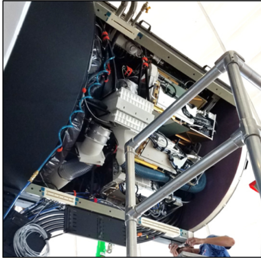
Figure 20. from Joseph Harry Silber et al 2023 Astron. J. 165 doi:10.3847/1538-3881/ac9ab1 https://dx.doi.org/10.3847/1538-3881/ac9ab1 © 2022. The Author(s). Published by the American Astronomical Society.
