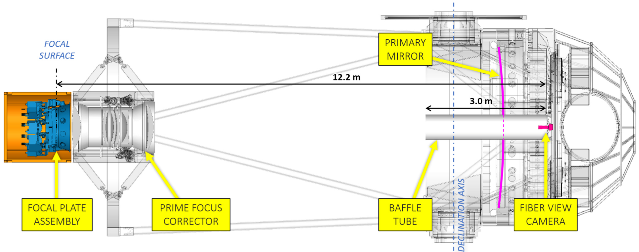
Figure 2. from Joseph Harry Silber et al 2023 Astron. J. 165 doi:10.3847/1538-3881/ac9ab1 https://dx.doi.org/10.3847/1538-3881/ac9ab1 © 2022. The Author(s). Published by the American Astronomical Society.
