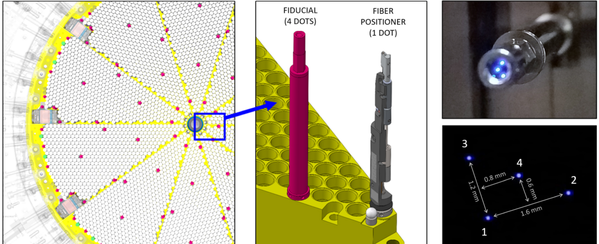
Figure 19. from Joseph Harry Silber et al 2023 Astron. J. 165 doi:10.3847/1538-3881/ac9ab1 https://dx.doi.org/10.3847/1538-3881/ac9ab1 © 2022. The Author(s). Published by the American Astronomical Society.
