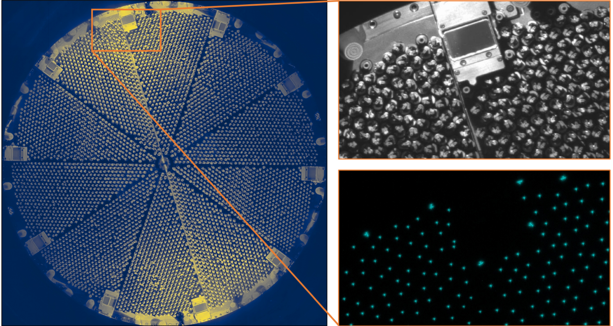
Figure 18. from Joseph Harry Silber et al 2023 Astron. J. 165 doi:10.3847/1538-3881/ac9ab1 https://dx.doi.org/10.3847/1538-3881/ac9ab1 © 2022. The Author(s). Published by the American Astronomical Society.
