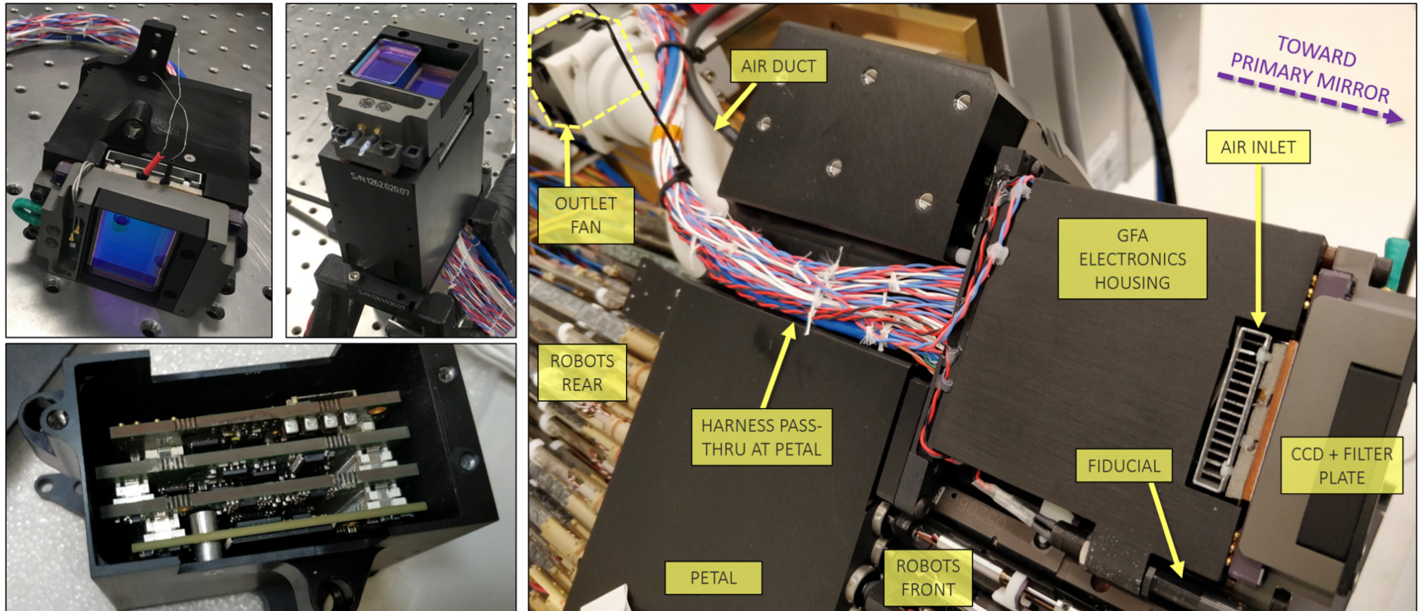
Figure 17. from Joseph Harry Silber et al 2023 Astron. J. 165 doi:10.3847/1538-3881/ac9ab1 https://dx.doi.org/10.3847/1538-3881/ac9ab1 © 2022. The Author(s). Published by the American Astronomical Society.
