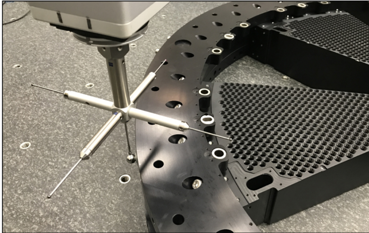
Figure 15. from Joseph Harry Silber et al 2023 Astron. J. 165 doi:10.3847/1538-3881/ac9ab1 https://dx.doi.org/10.3847/1538-3881/ac9ab1 © 2022. The Author(s). Published by the American Astronomical Society.
