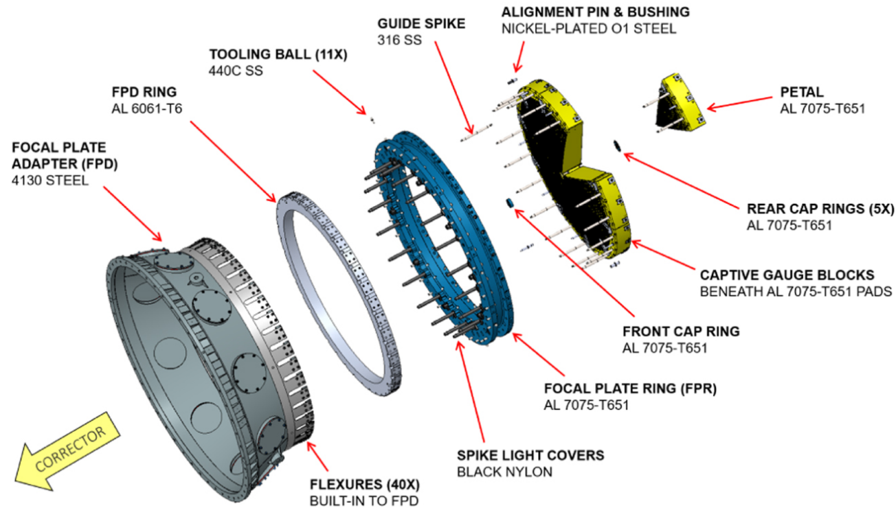
Figure 14. from Joseph Harry Silber et al 2023 Astron. J. 165 doi:10.3847/1538-3881/ac9ab1 https://dx.doi.org/10.3847/1538-3881/ac9ab1 © 2022. The Author(s). Published by the American Astronomical Society.
