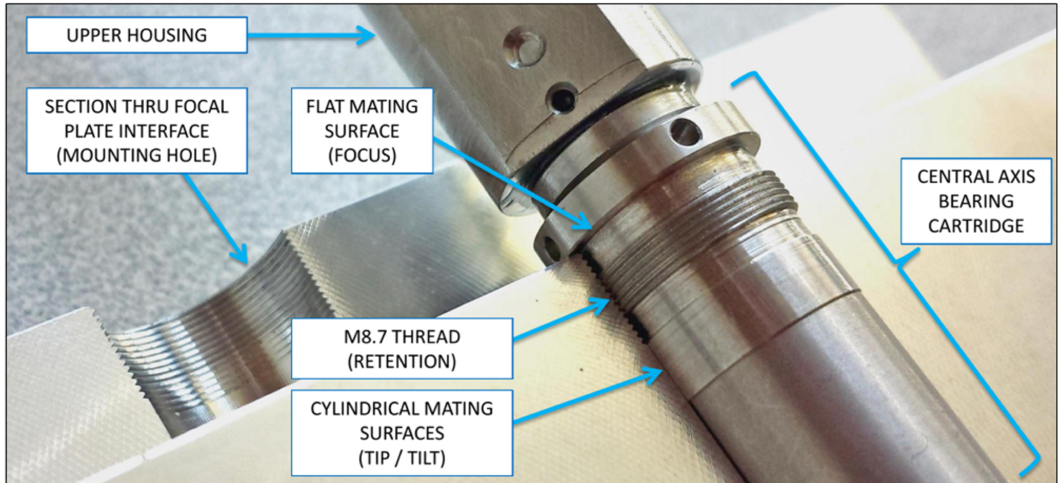
Figure 12. from Joseph Harry Silber et al 2023 Astron. J. 165 doi:10.3847/1538-3881/ac9ab1 https://dx.doi.org/10.3847/1538-3881/ac9ab1 © 2022. The Author(s). Published by the American Astronomical Society.
