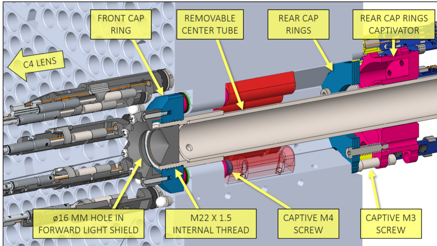
Figure 11. from Joseph Harry Silber et al 2023 Astron. J. 165 doi:10.3847/1538-3881/ac9ab1 https://dx.doi.org/10.3847/1538-3881/ac9ab1 © 2022. The Author(s). Published by the American Astronomical Society.
