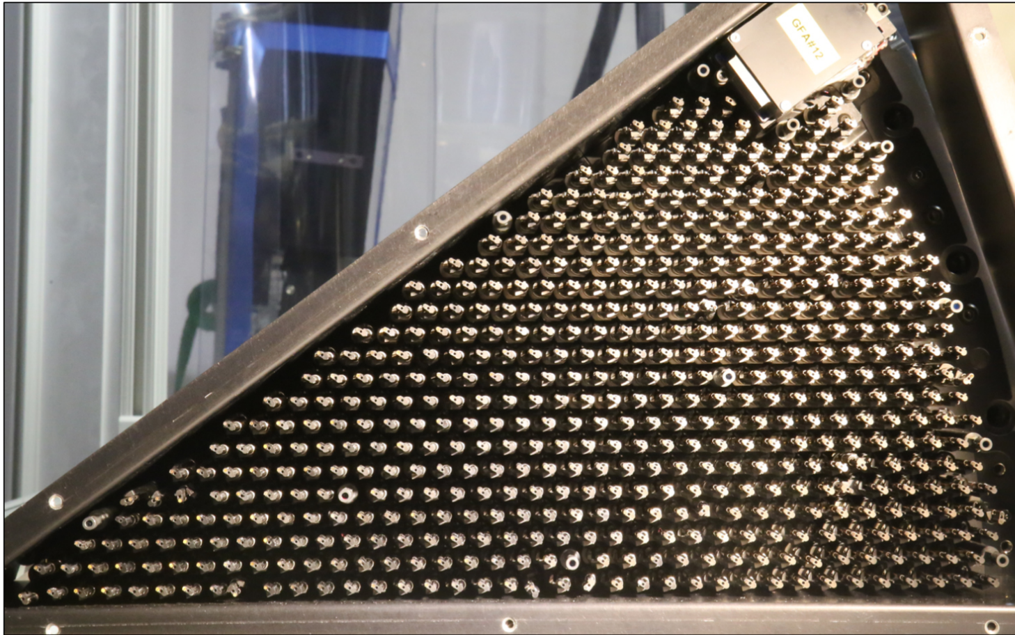
Figure 1. from Joseph Harry Silber et al 2023 Astron. J. 165 doi:10.3847/1538-3881/ac9ab1 https://dx.doi.org/10.3847/1538-3881/ac9ab1 © 2022. The Author(s). Published by the American Astronomical Society.
