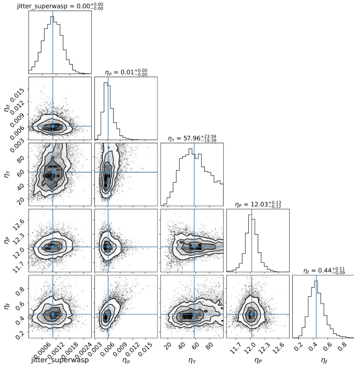
Figure 9. from Mohammed El Mufti et al 2023 Astron. J. 165 doi:10.3847/1538-3881/ac9834 https://dx.doi.org/10.3847/1538-3881/ac9834 © 2022. The Author(s). Published by the American Astronomical Society.
