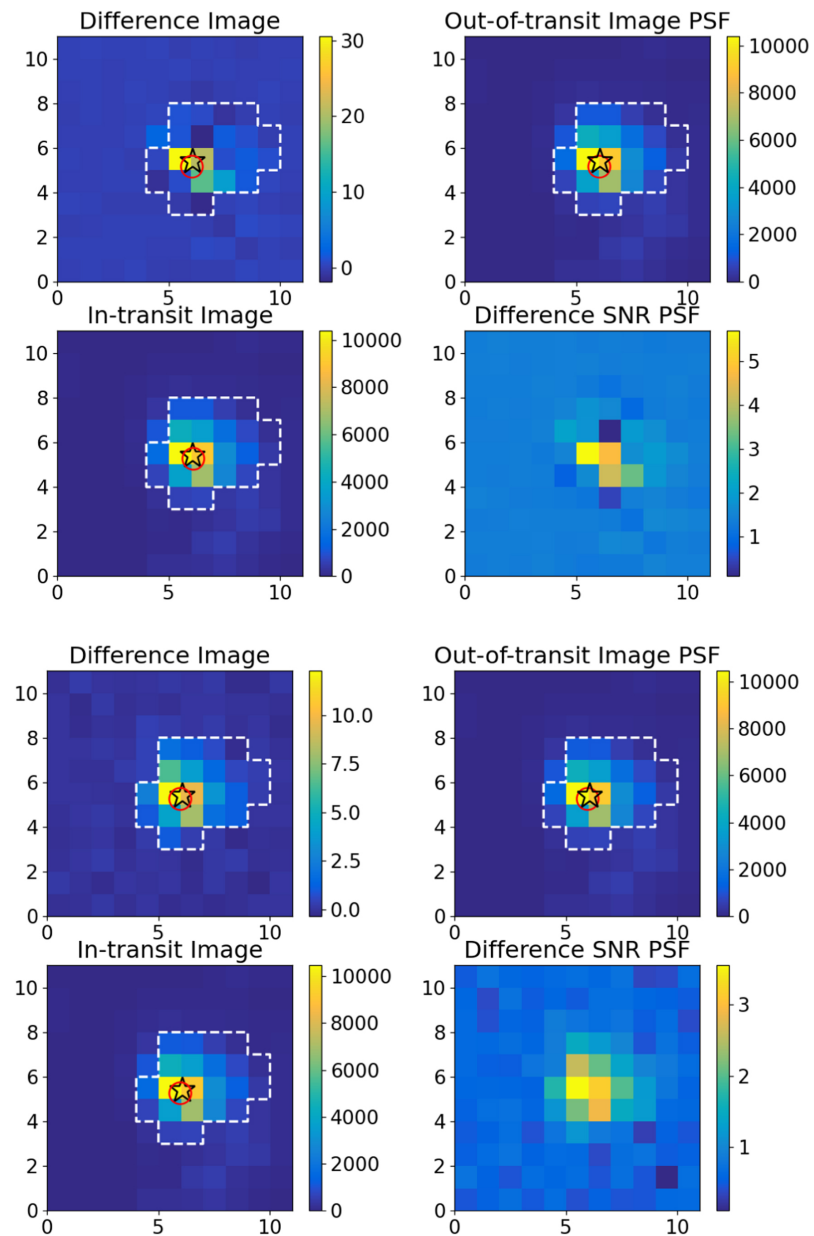
Figure 40. from Mohammed El Mufti et al 2023 Astron. J. 165 doi:10.3847/1538-3881/ac9834 https://dx.doi.org/10.3847/1538-3881/ac9834 © 2022. The Author(s). Published by the American Astronomical Society.
