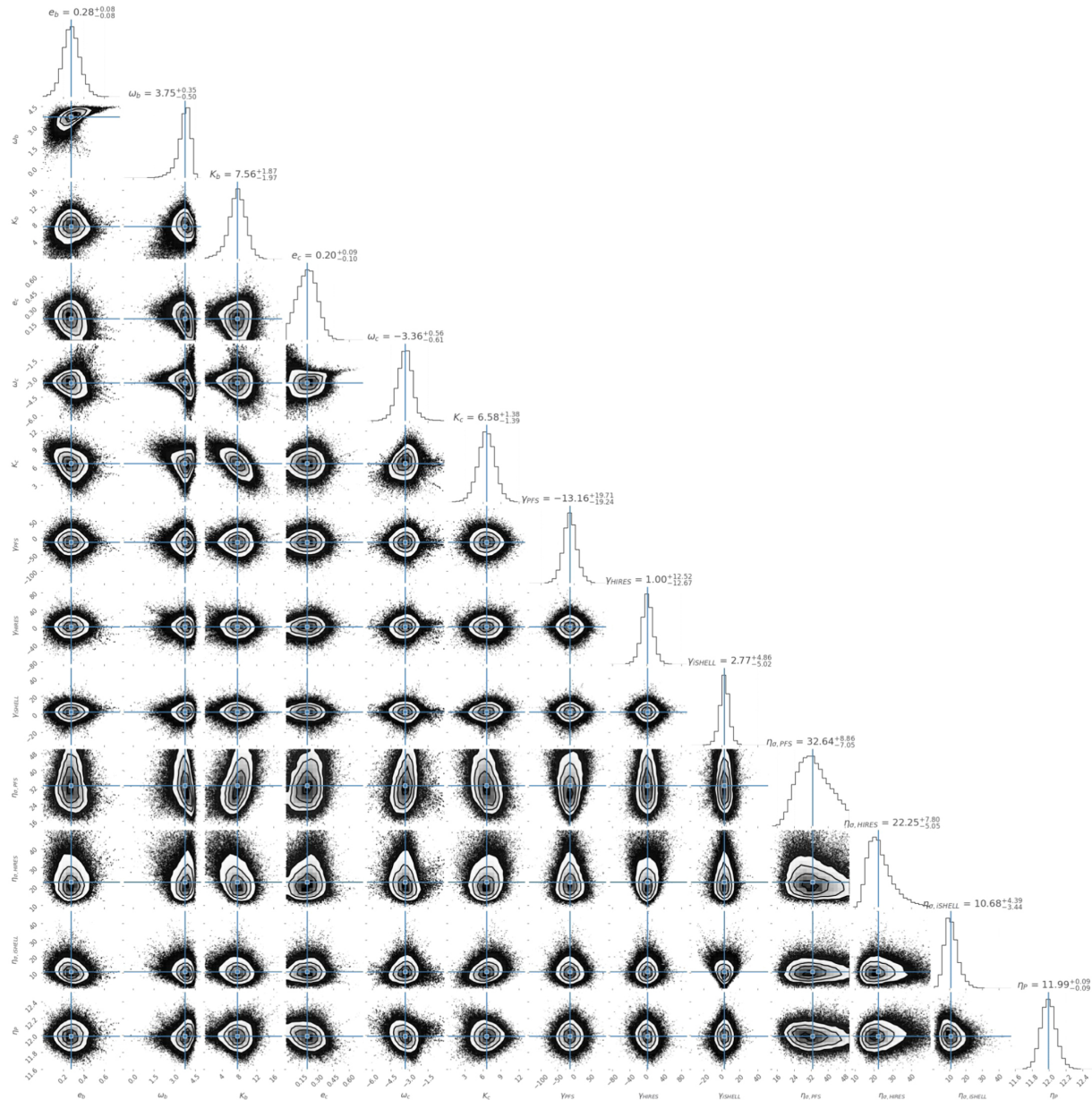
Figure 37. from Mohammed El Mufti et al 2023 Astron. J. 165 doi:10.3847/1538-3881/ac9834 https://dx.doi.org/10.3847/1538-3881/ac9834 © 2022. The Author(s). Published by the American Astronomical Society.
