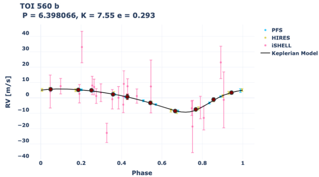
Figure 36. from Mohammed El Mufti et al 2023 Astron. J. 165 doi:10.3847/1538-3881/ac9834 https://dx.doi.org/10.3847/1538-3881/ac9834 © 2022. The Author(s). Published by the American Astronomical Society.
