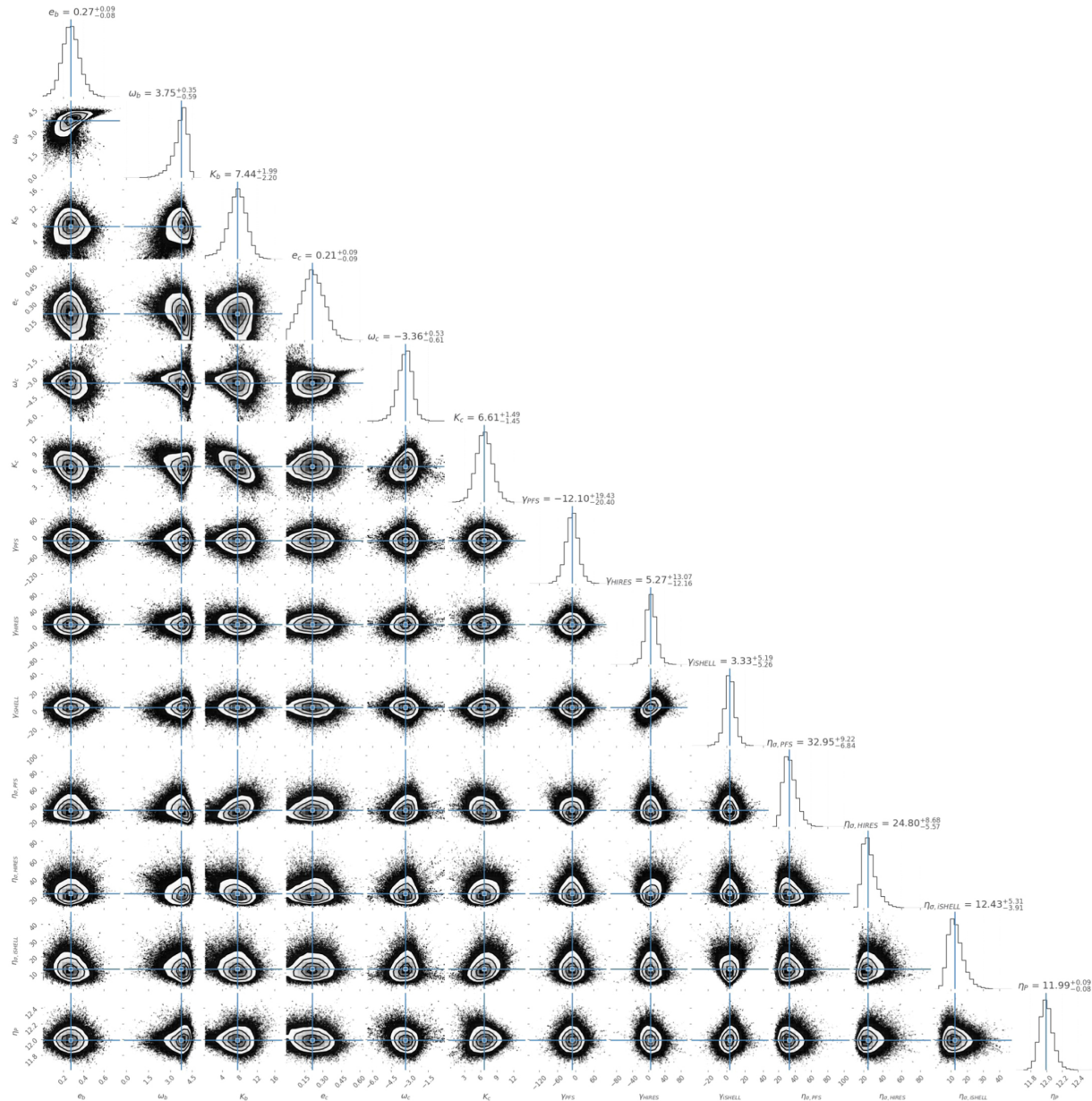
Figure 34. from Mohammed El Mufti et al 2023 Astron. J. 165 doi:10.3847/1538-3881/ac9834 https://dx.doi.org/10.3847/1538-3881/ac9834 © 2022. The Author(s). Published by the American Astronomical Society.
