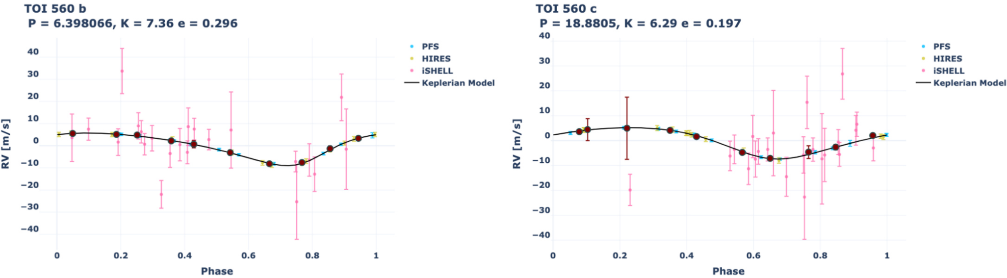
Figure 33. from Mohammed El Mufti et al 2023 Astron. J. 165 doi:10.3847/1538-3881/ac9834 https://dx.doi.org/10.3847/1538-3881/ac9834 © 2022. The Author(s). Published by the American Astronomical Society.
