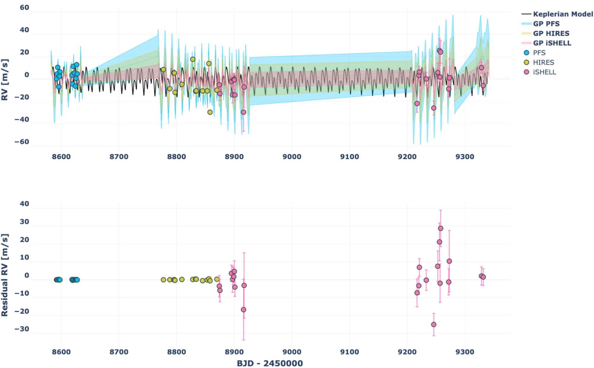
Figure 32. from Mohammed El Mufti et al 2023 Astron. J. 165 doi:10.3847/1538-3881/ac9834 https://dx.doi.org/10.3847/1538-3881/ac9834 © 2022. The Author(s). Published by the American Astronomical Society.
