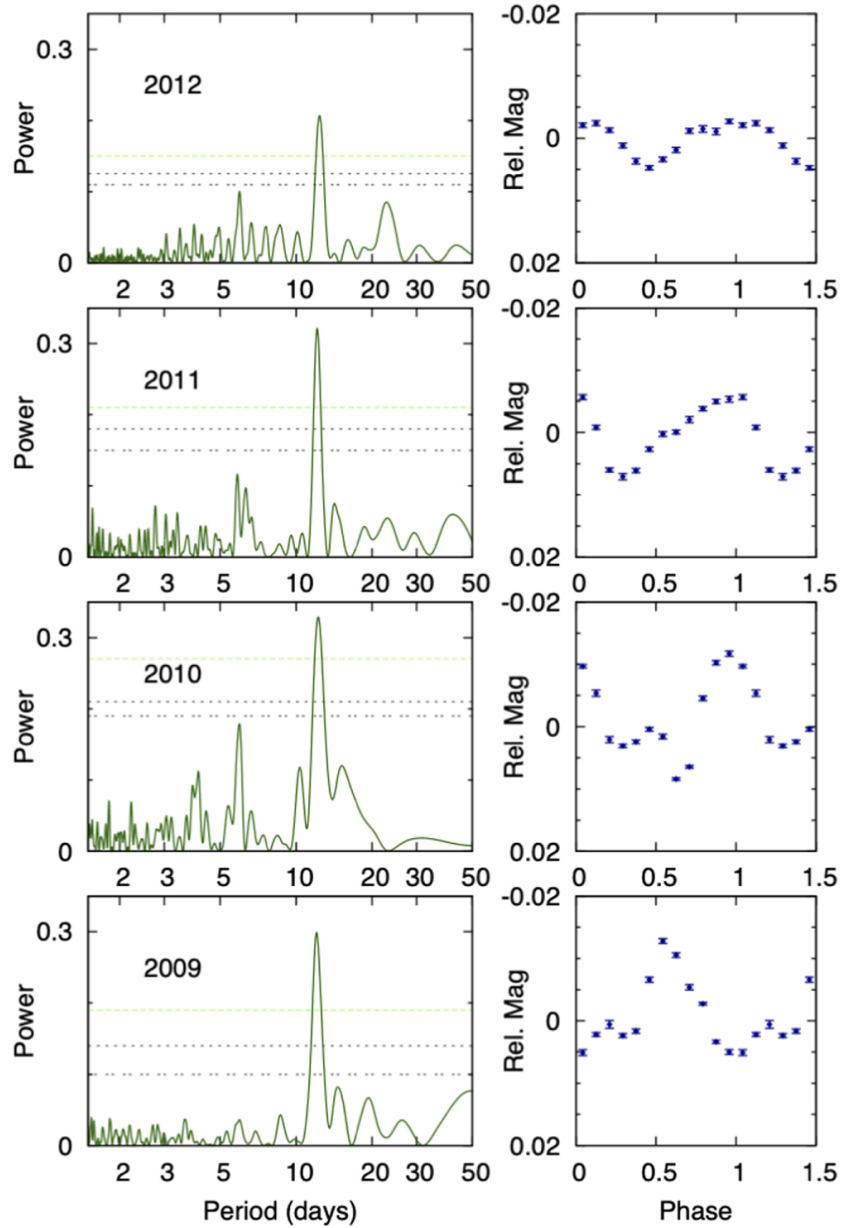
Figure 3. from Mohammed El Mufti et al 2023 Astron. J. 165 doi:10.3847/1538-3881/ac9834 https://dx.doi.org/10.3847/1538-3881/ac9834 © 2022. The Author(s). Published by the American Astronomical Society.
