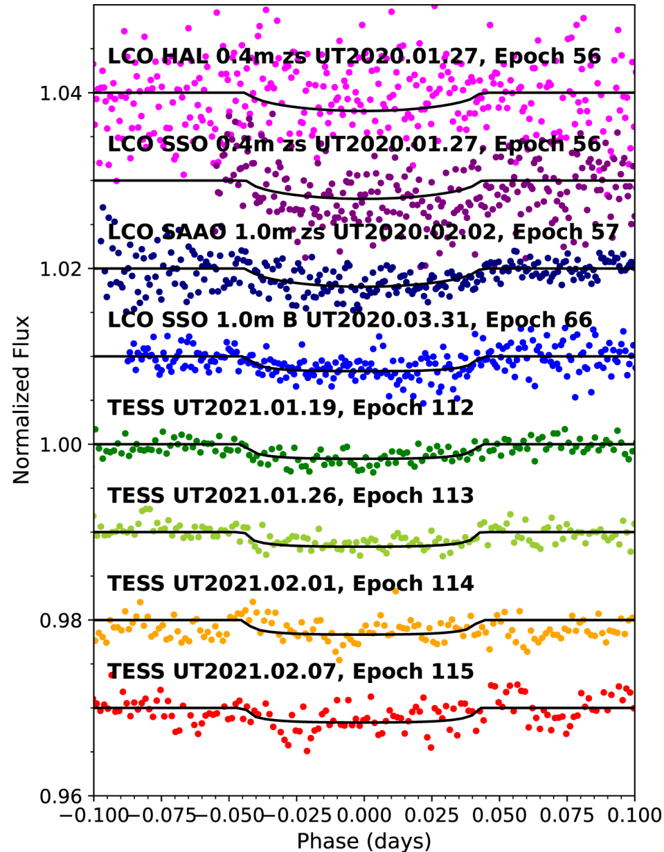
Figure 27. from Mohammed El Mufti et al 2023 Astron. J. 165 doi:10.3847/1538-3881/ac9834 https://dx.doi.org/10.3847/1538-3881/ac9834 © 2022. The Author(s). Published by the American Astronomical Society.
