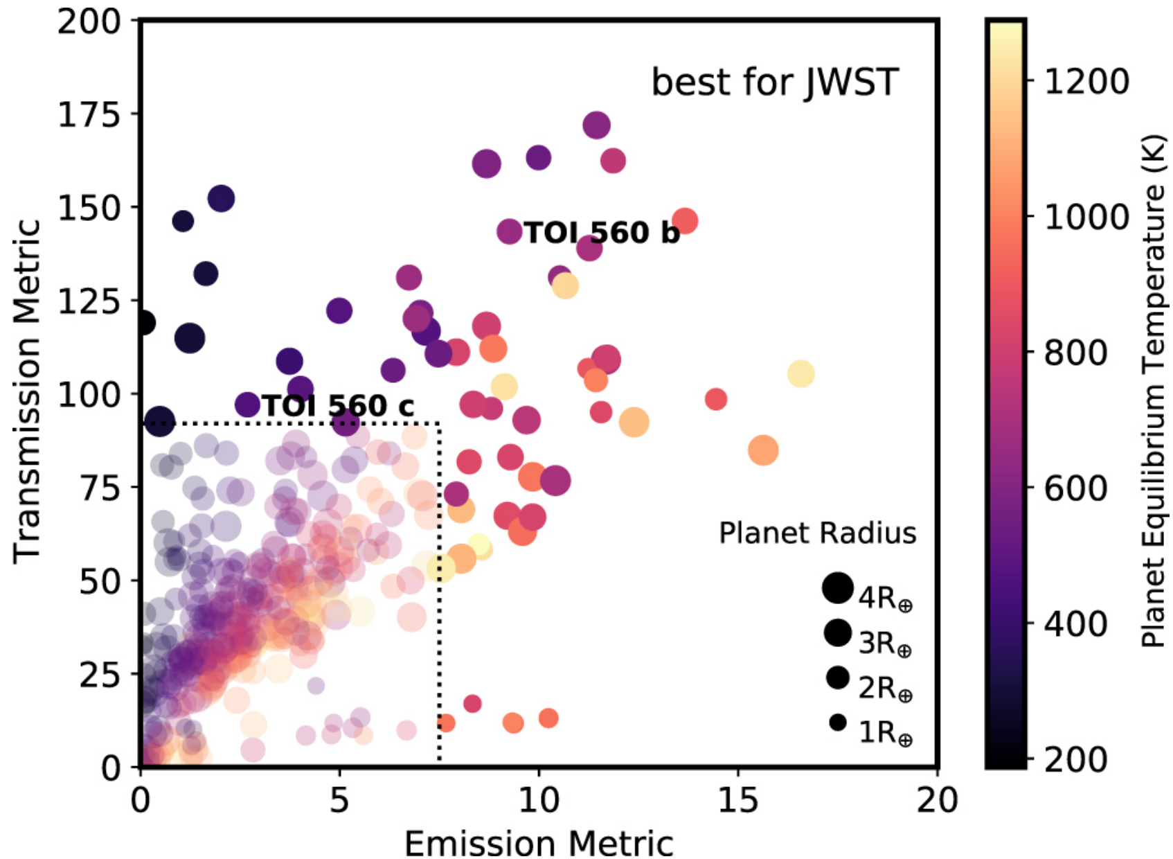
Figure 24. from Mohammed El Mufti et al 2023 Astron. J. 165 doi:10.3847/1538-3881/ac9834 https://dx.doi.org/10.3847/1538-3881/ac9834 © 2022. The Author(s). Published by the American Astronomical Society.
