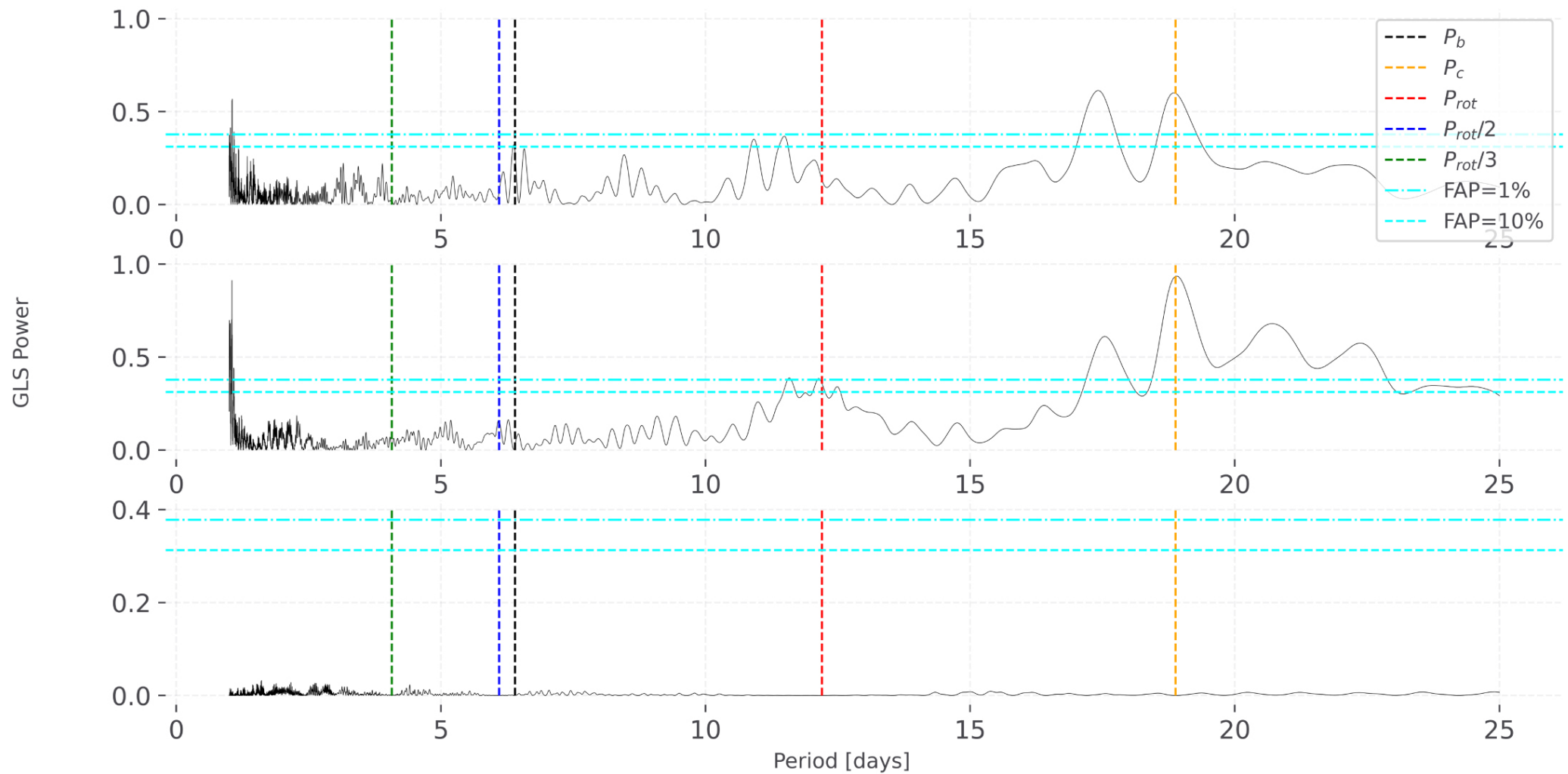
Figure 22. from Mohammed El Mufti et al 2023 Astron. J. 165 doi:10.3847/1538-3881/ac9834 https://dx.doi.org/10.3847/1538-3881/ac9834 © 2022. The Author(s). Published by the American Astronomical Society.
