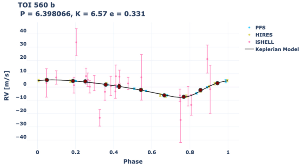
Figure 18. from Mohammed El Mufti et al 2023 Astron. J. 165 doi:10.3847/1538-3881/ac9834 https://dx.doi.org/10.3847/1538-3881/ac9834 © 2022. The Author(s). Published by the American Astronomical Society.
