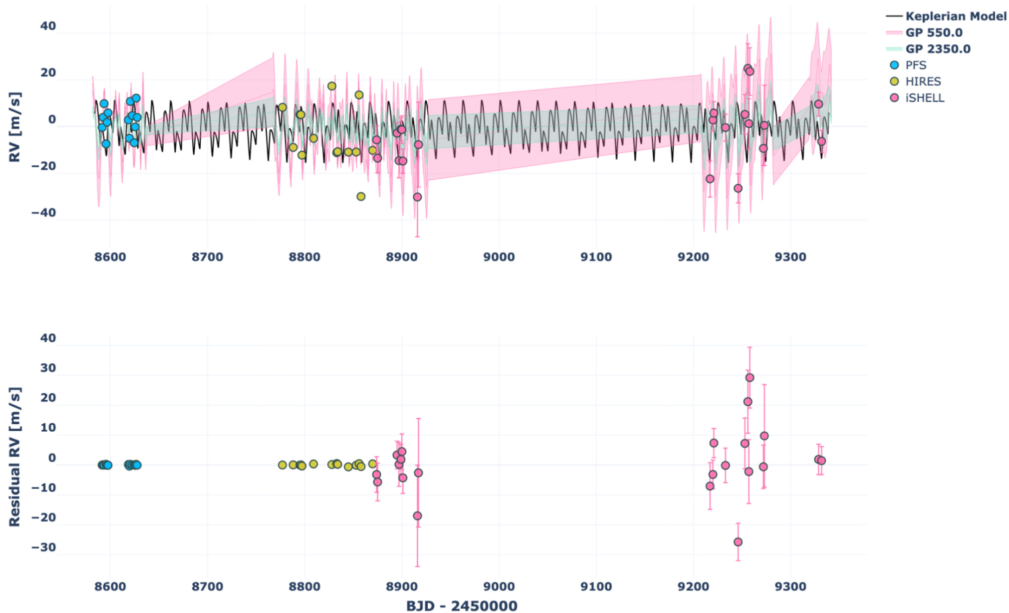
Figure 17. from Mohammed El Mufti et al 2023 Astron. J. 165 doi:10.3847/1538-3881/ac9834 https://dx.doi.org/10.3847/1538-3881/ac9834 © 2022. The Author(s). Published by the American Astronomical Society.
