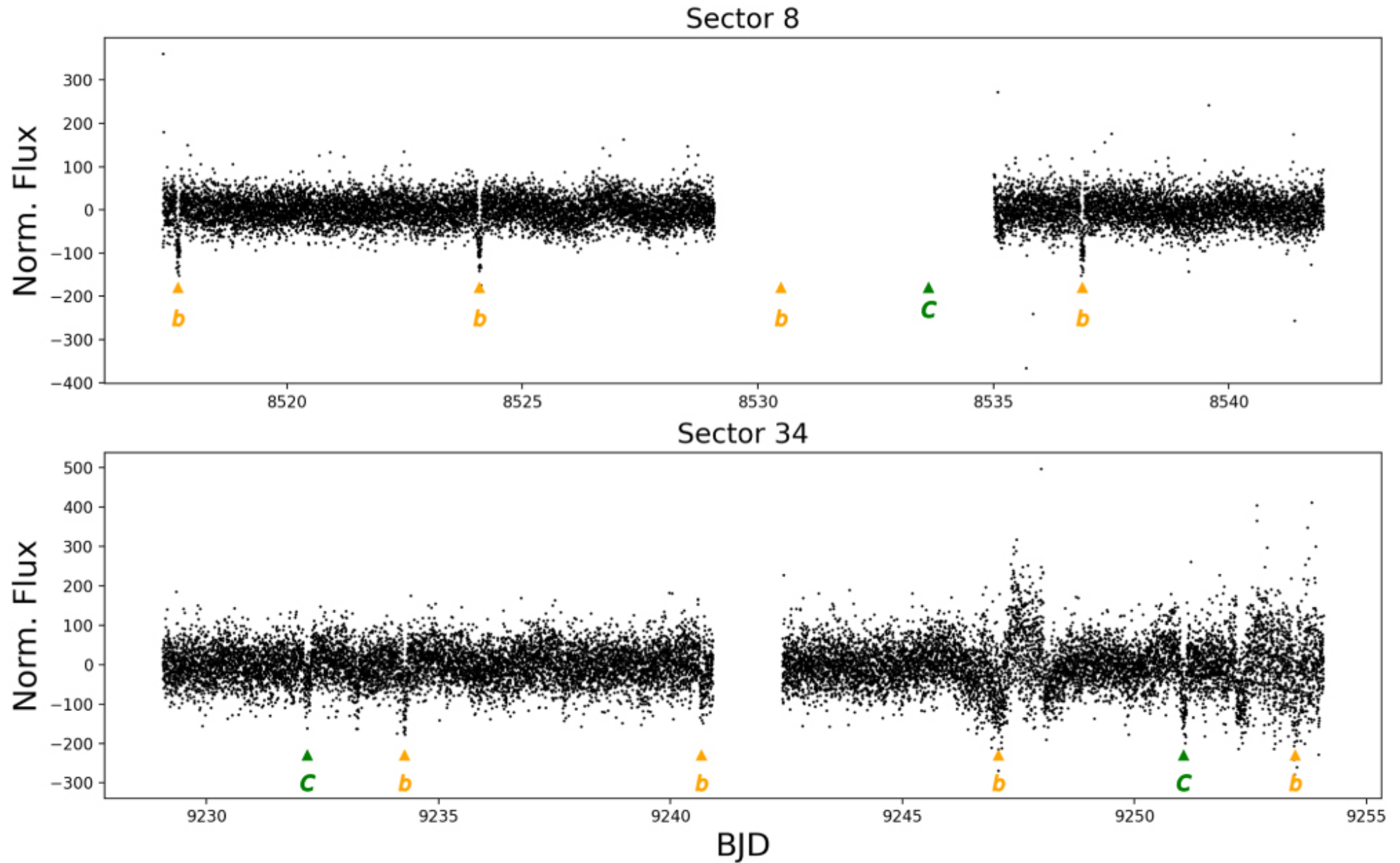
Figure 13. from Mohammed El Mufti et al 2023 Astron. J. 165 doi:10.3847/1538-3881/ac9834 https://dx.doi.org/10.3847/1538-3881/ac9834 © 2022. The Author(s). Published by the American Astronomical Society.
