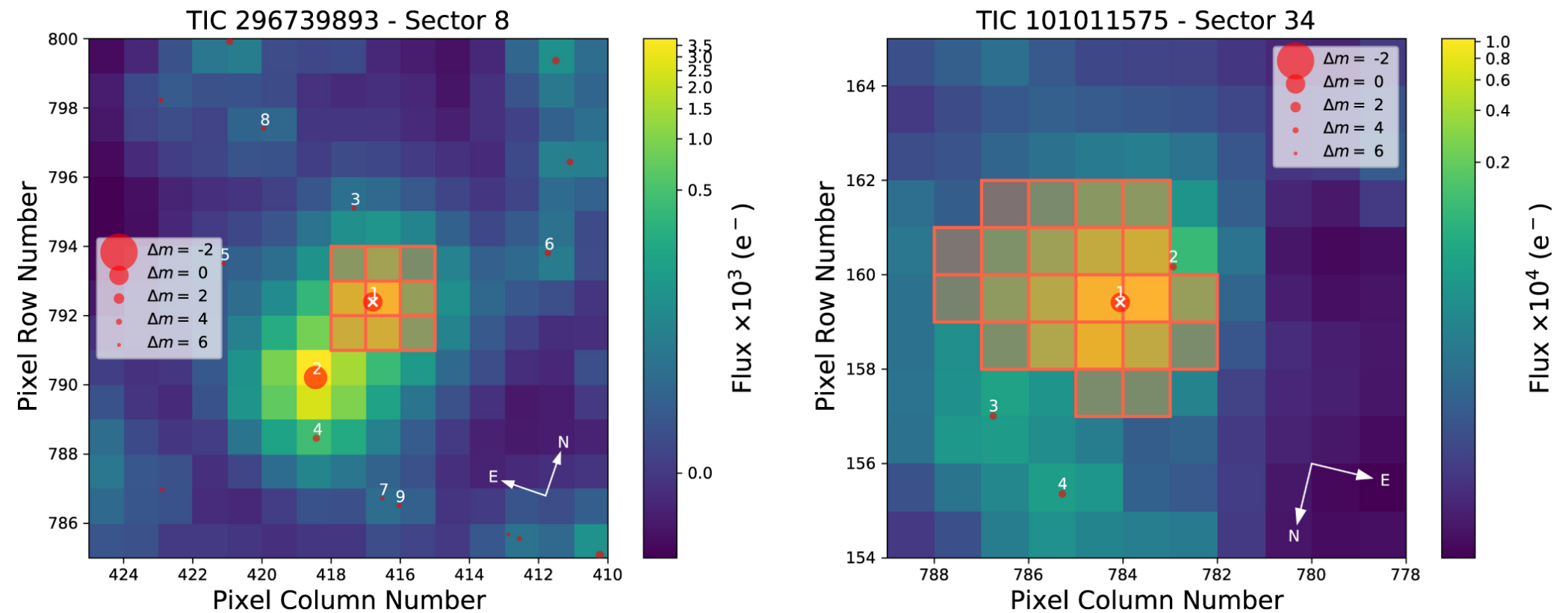
Figure 1. from Mohammed El Mufti et al 2023 Astron. J. 165 doi:10.3847/1538-3881/ac9834 https://dx.doi.org/10.3847/1538-3881/ac9834 © 2022. The Author(s). Published by the American Astronomical Society.
