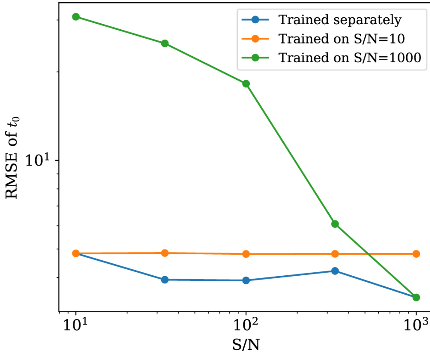
Figure 8. from Haimeng Zhao et al 2022 Astron. J. 164 doi:10.3847/1538-3881/ac9230 https://dx.doi.org/10.3847/1538-3881/ac9230 © 2022. The Author(s). Published by the American Astronomical Society.
