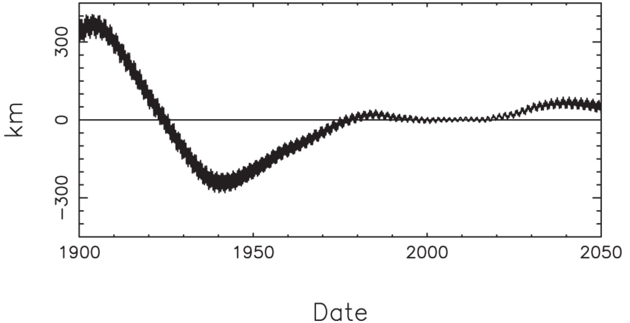
Figure 9. from Robert. A. Jacobson 2022 Astron. J. 164 doi:10.3847/1538-3881/ac90c9 https://dx.doi.org/10.3847/1538-3881/ac90c9 © 2022. The Author(s). Published by the American Astronomical Society.
