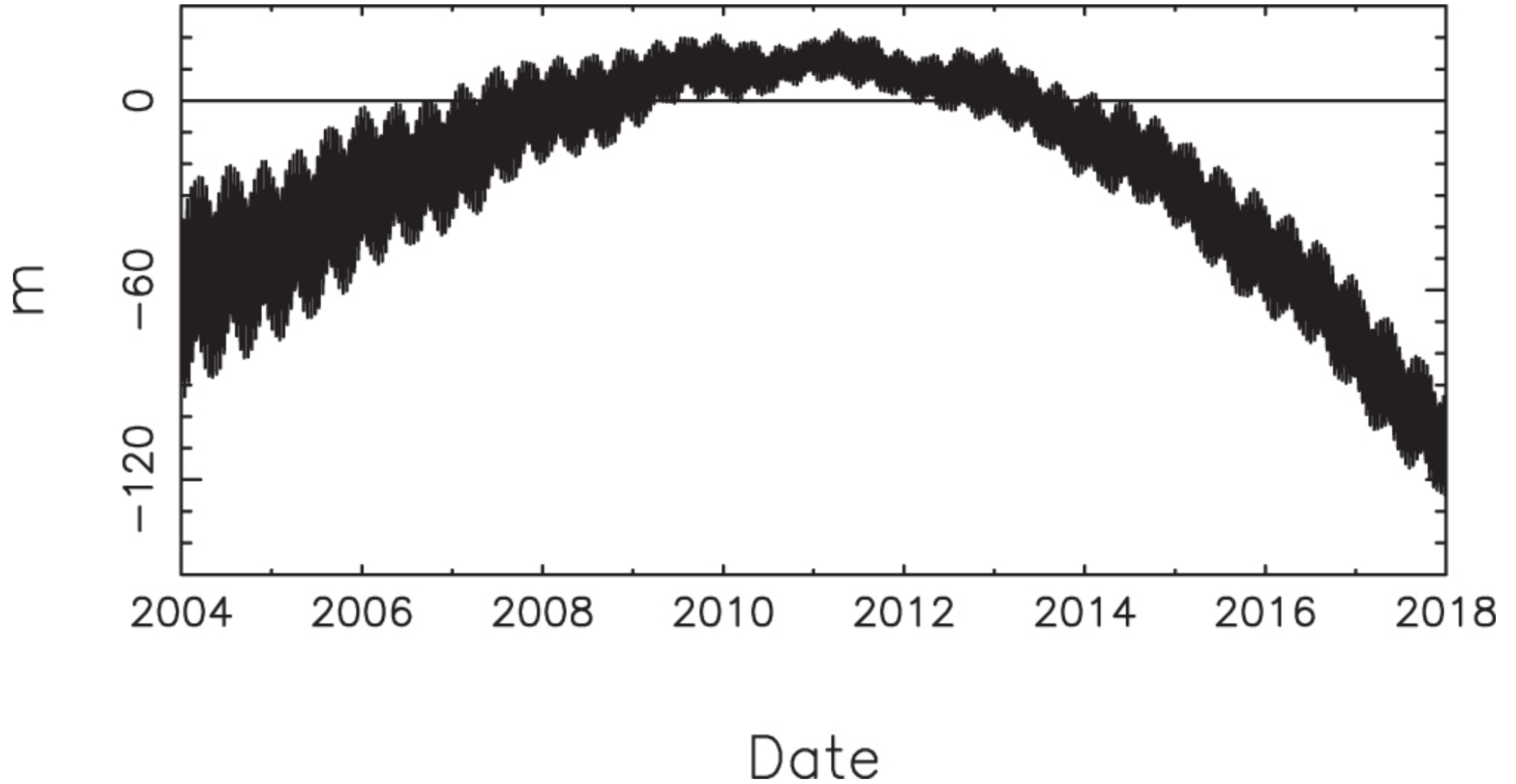
Figure 6. from Robert. A. Jacobson 2022 Astron. J. 164 doi:10.3847/1538-3881/ac90c9 https://dx.doi.org/10.3847/1538-3881/ac90c9 © 2022. The Author(s). Published by the American Astronomical Society.
