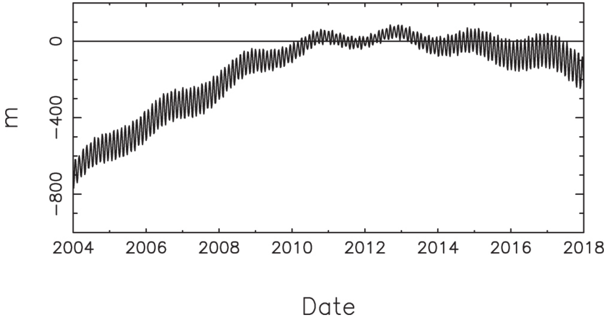
Figure 4. from Robert. A. Jacobson 2022 Astron. J. 164 doi:10.3847/1538-3881/ac90c9 https://dx.doi.org/10.3847/1538-3881/ac90c9 © 2022. The Author(s). Published by the American Astronomical Society.
