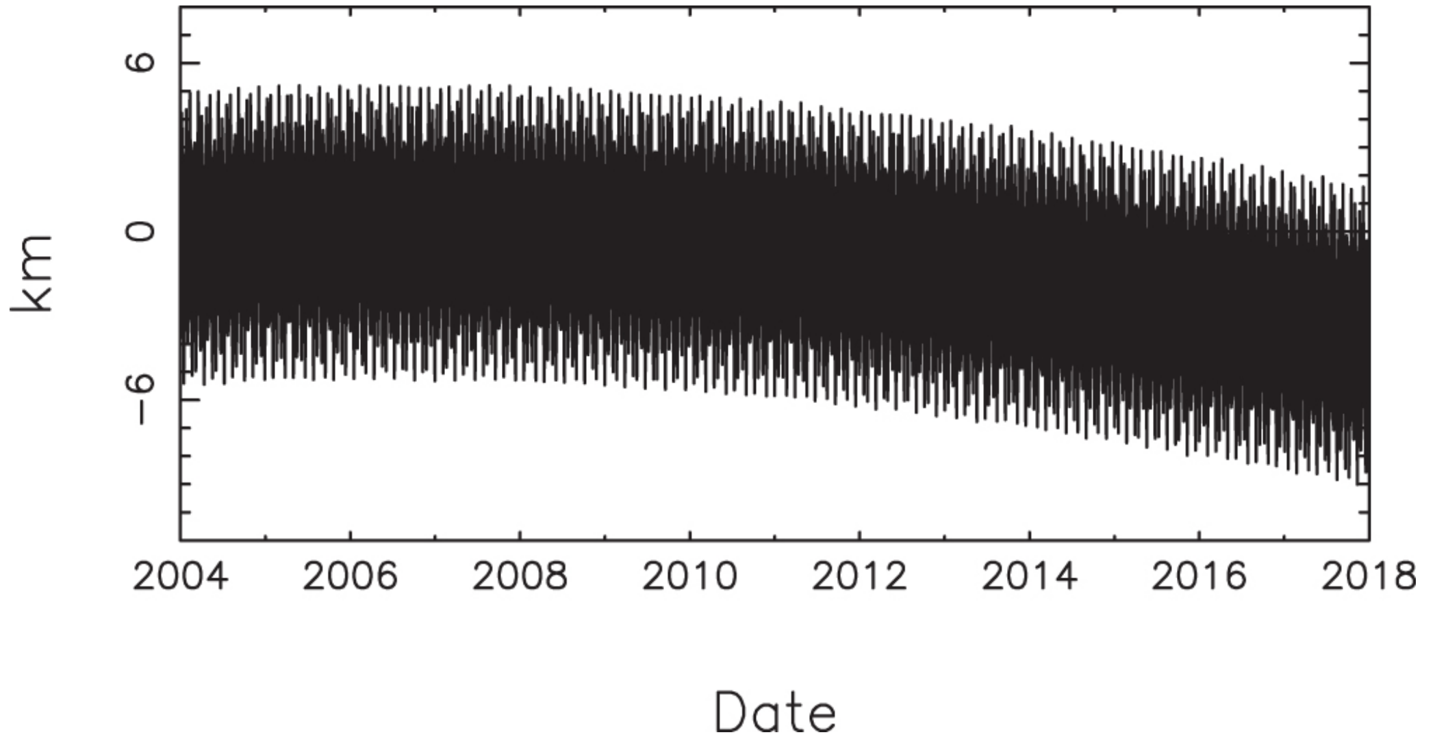
Figure 3. from Robert. A. Jacobson 2022 Astron. J. 164 doi:10.3847/1538-3881/ac90c9 https://dx.doi.org/10.3847/1538-3881/ac90c9 © 2022. The Author(s). Published by the American Astronomical Society.
